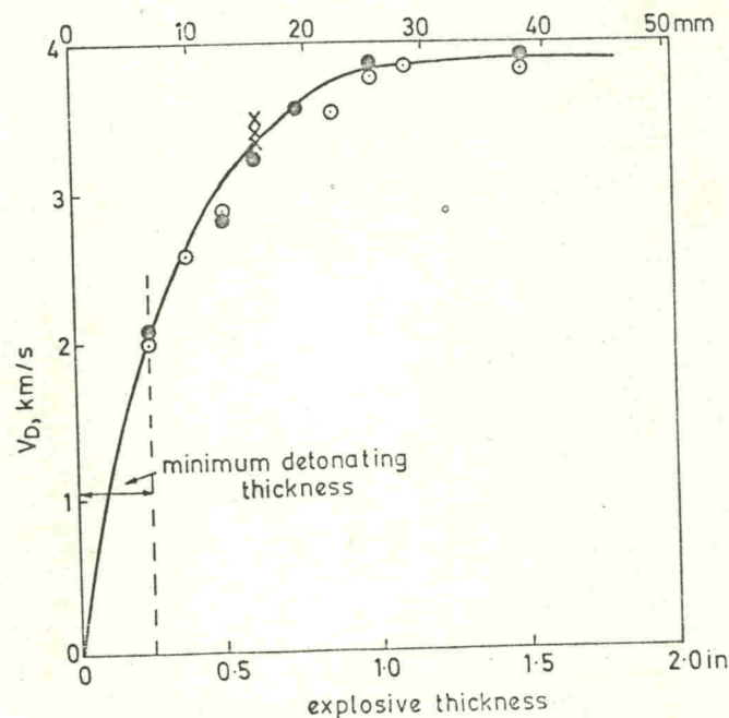
9 Effect of thickness of layer of Trimonite No. 3 on the detonation velocity. \rho = 0.98 g/cm 3 . ○ Dautriche × parallel plate ● pin insertion
